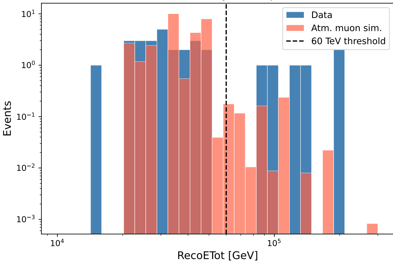
Data vs. simulation (sim scaled by full-sample ratio 3.82 \pm 1.59 )
