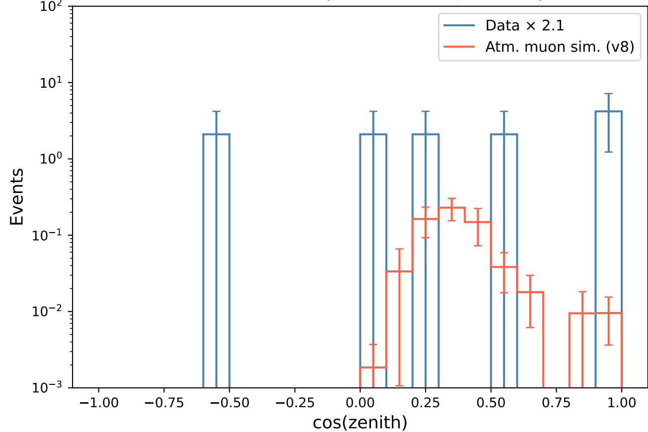
Zenith — &gt;60 TeV (data×2.1 vs. v8, unscaled)
