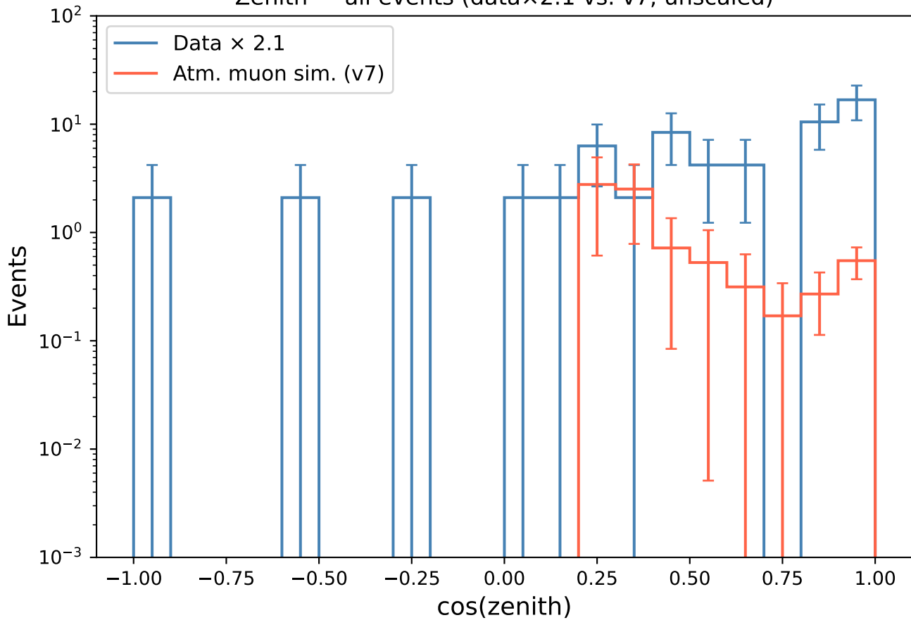
Zenith — all events (data \times 2.1 vs. v7, unscaled)
