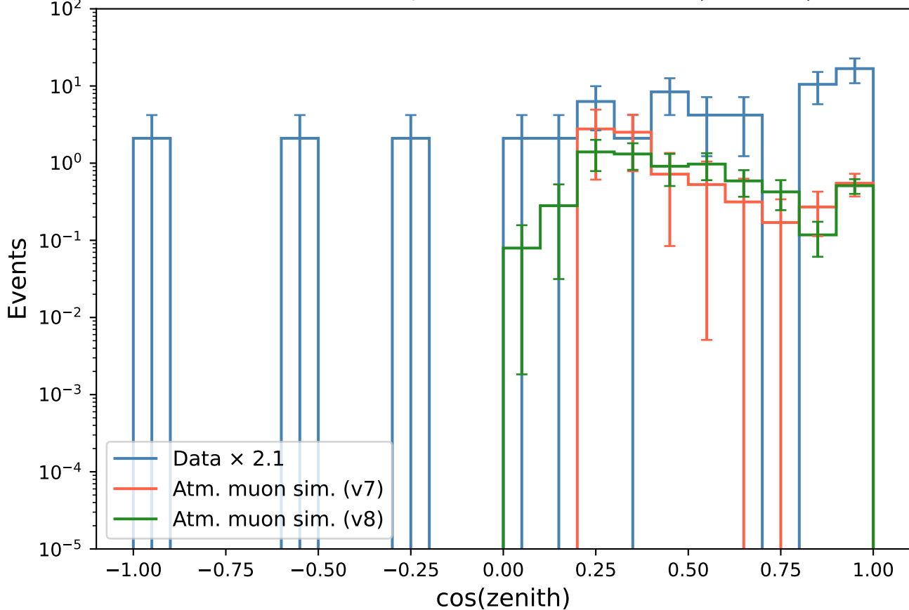
Zenith — all events, data \times 2.1 vs. v7 and v8 (unscaled)
