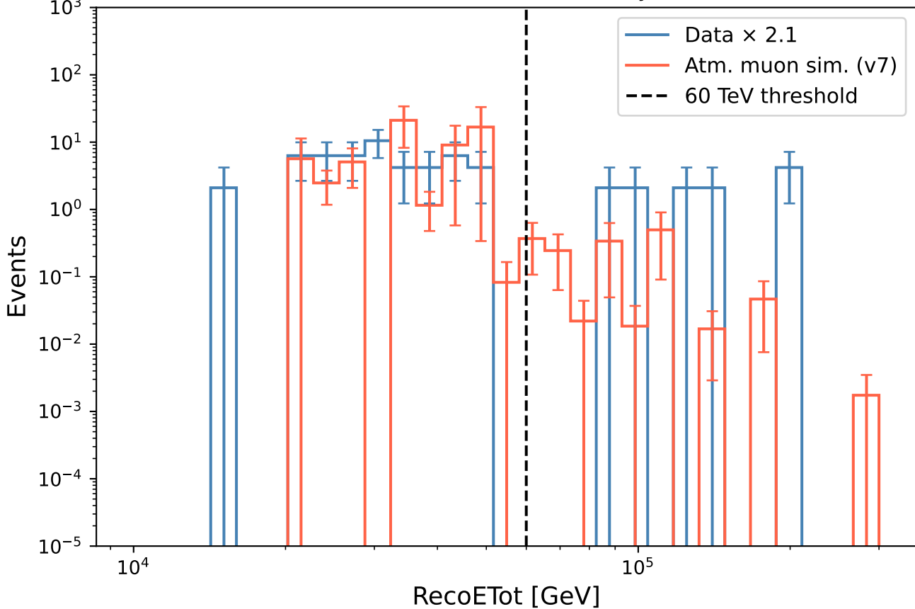
Data \times 2.1 vs. simulation (v7, scaled by 8.03 \pm 3.33 )
