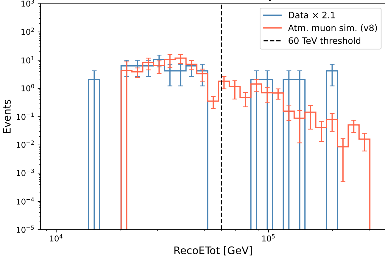
Data \times 2.1 vs. simulation (v8, scaled by 9.55 \pm 2.30 )
