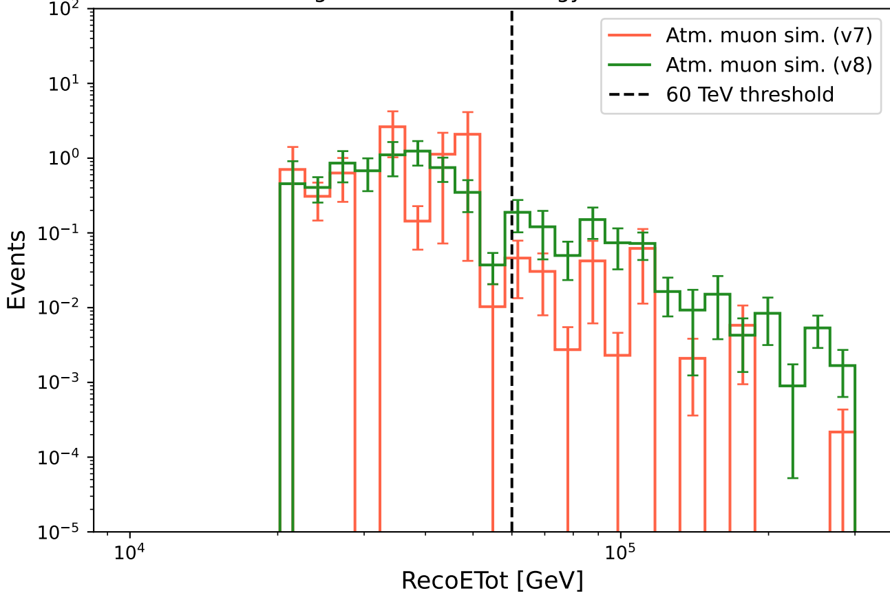
Weighted simulation energy — v7 vs v8
