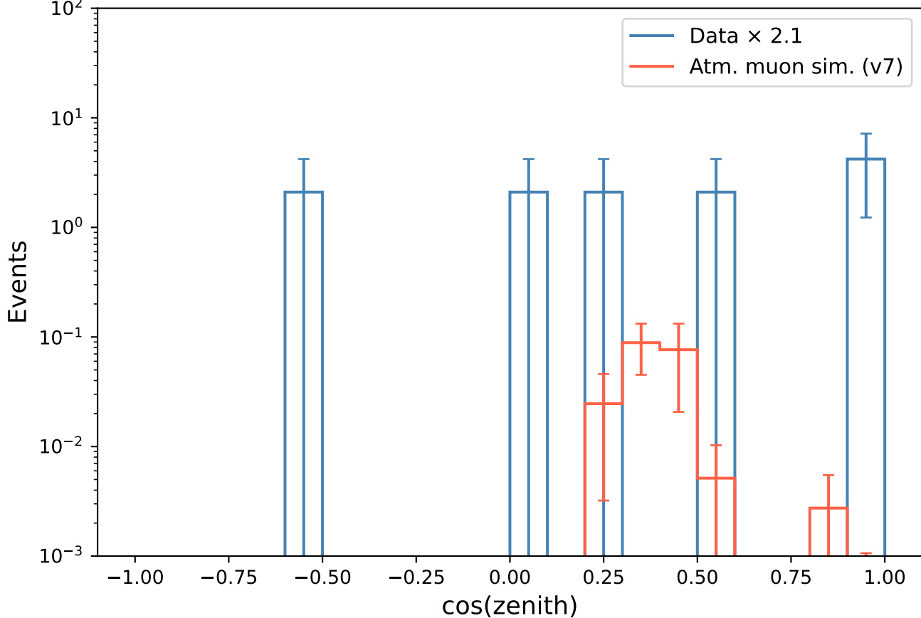
Zenith — >60 TeV (data \times 2.1 vs. v7, unscaled)
