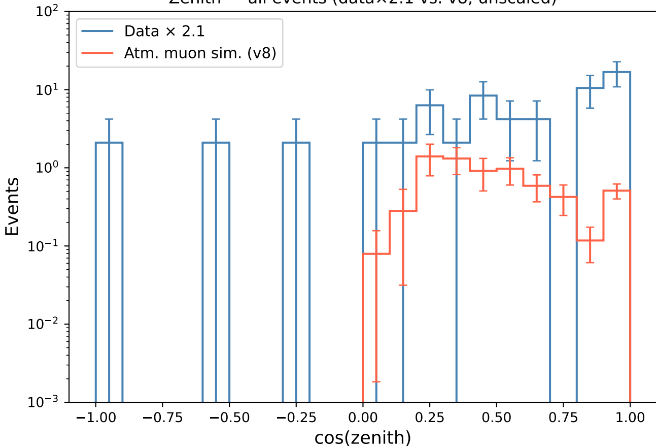
Zenith — all events (data \times 2.1 vs. v8, unscaled)
