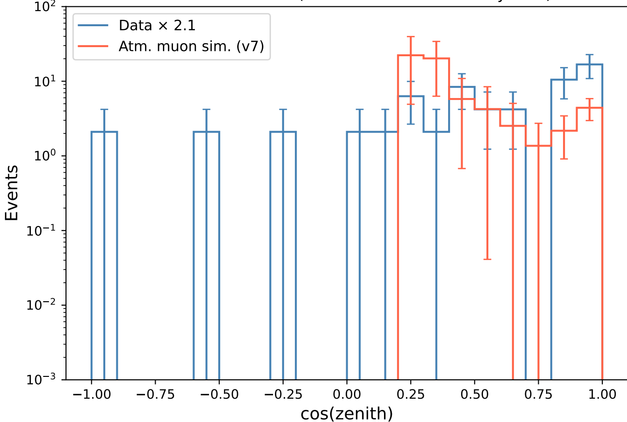
Zenith — all events (data \times 2.1 vs. v7 scaled by 8.03)
