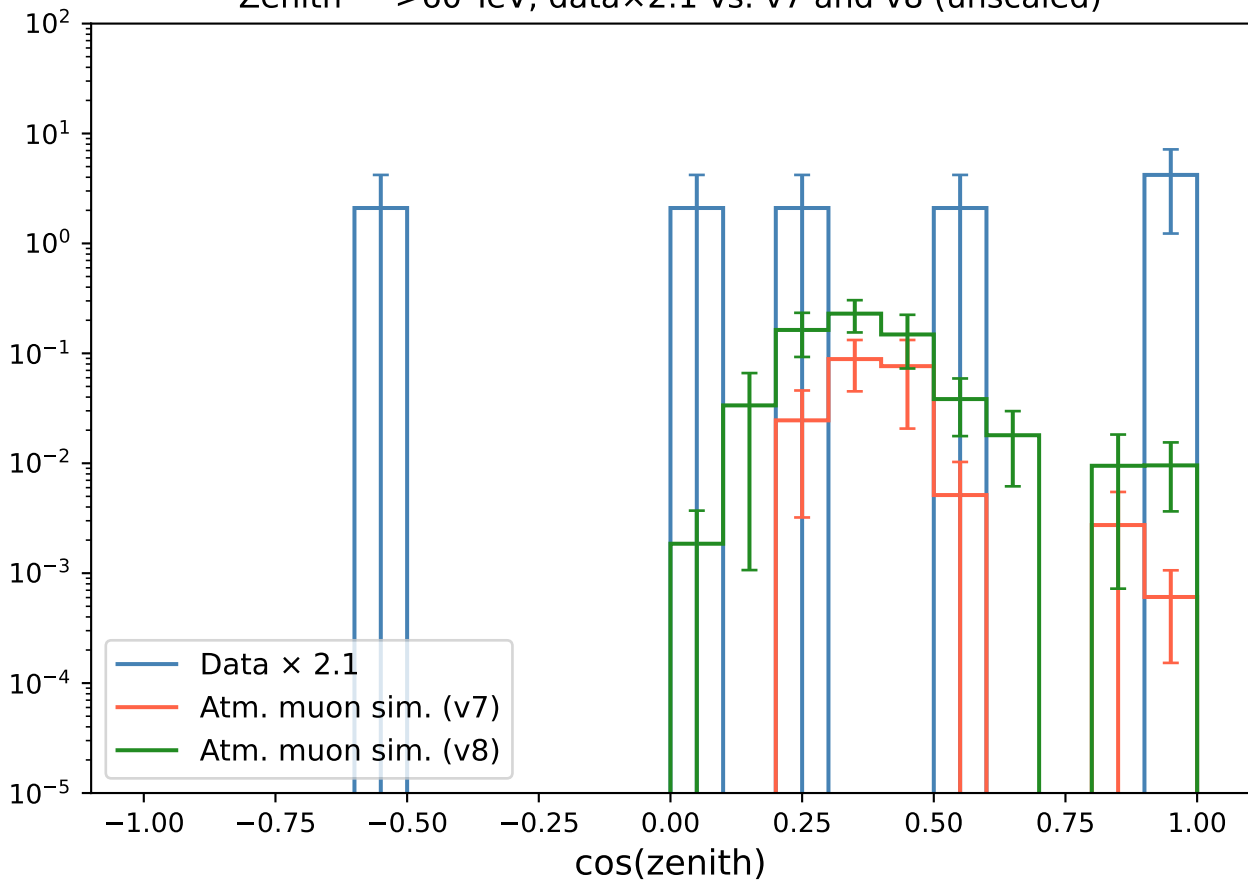
Zenith — &gt;60 TeV, data×2.1 vs. v7 and v8 (unscaled)
