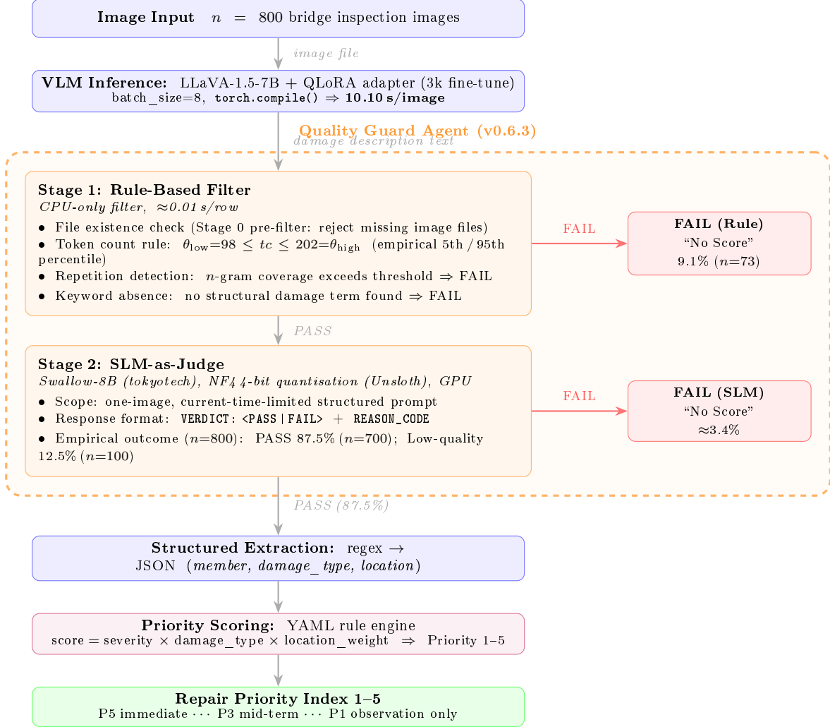
Figure 11: Complete algorithm flow of the Visual Inspection ScoreBot v0.6.3 pipeline. The Quality Guard Agent interposes between VLM inference and priority scoring, filtering low-quality outputs via a two-stage architecture: Stage 1 (rule-based, CPU, ≈0.01 s/row) and Stage 2 (Swallow-8B SLM judge, GPU, ≈10 s/row). Only outputs passing both stages receive a five-level Repair Priority Index; 12.5% of predictions are rejected as low quality.
