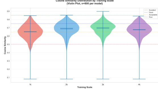
Figure 6: Violin plots of cosine similarity distributions. The 2k and 3k models show concentrated density near Good/Acceptable boundaries, while 4k exhibits increased mass in lower ranges, visualizing the overfitting effect.
