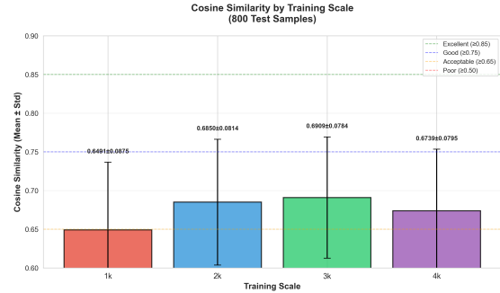
Figure 4: Cosine similarity comparison (1k–4k). Error bars represent standard deviation. Horizontal lines mark quality tier boundaries. The 3k model achieves peak performance (0.6909) before 4k degradation.
