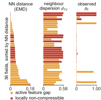
f Nearest-neighbour response panel
