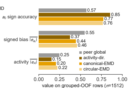
f Nearest-neighbour response panel
