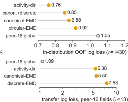
h Peer-16-only robustness
