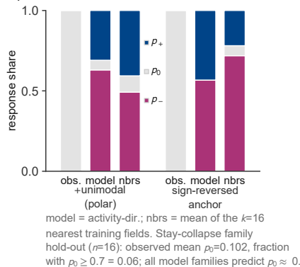
h Peer-16-only robustness
