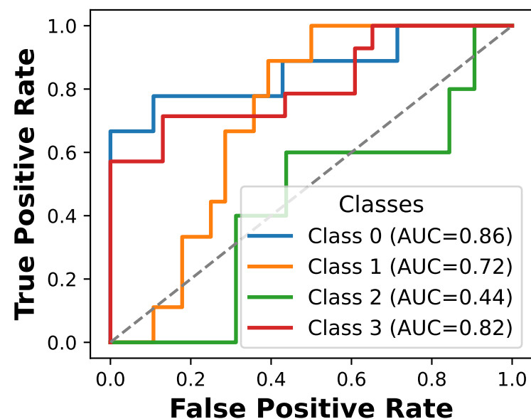
Ensemble ROC
