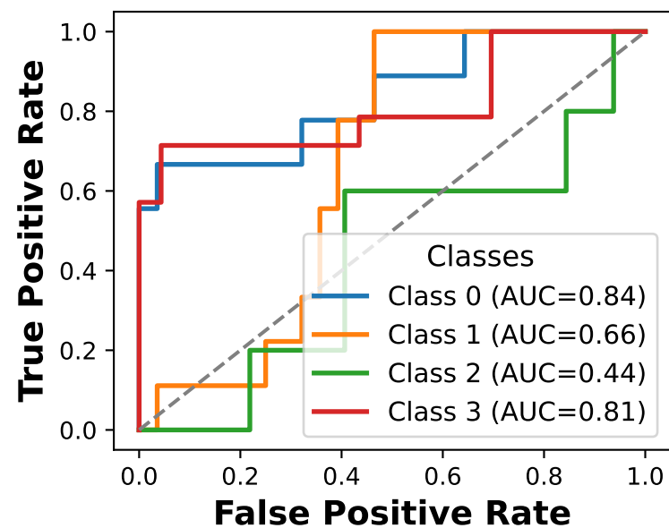
Ensemble ROC
