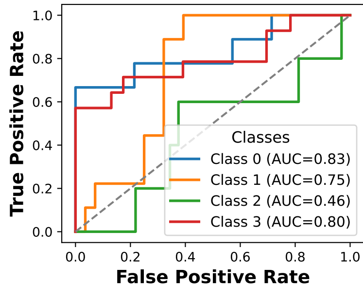
Neural Network ROC
