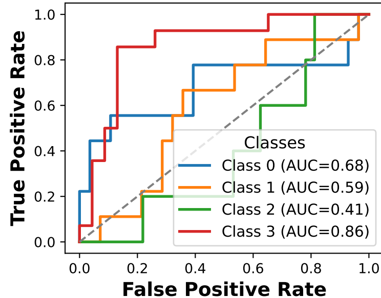
Neural Network ROC (ROS + IQR)
