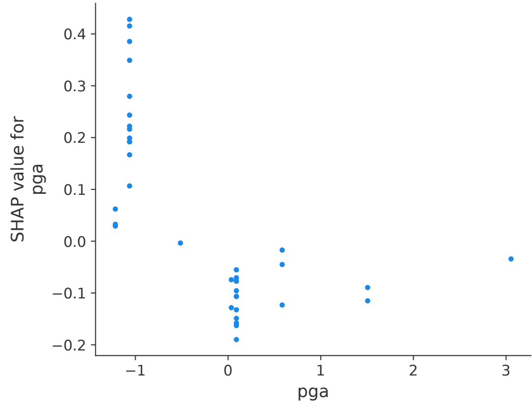
SHAP dependence (Class=3): PGA vs SHAP value (Gradient Boosting) (KernelSHAP)
