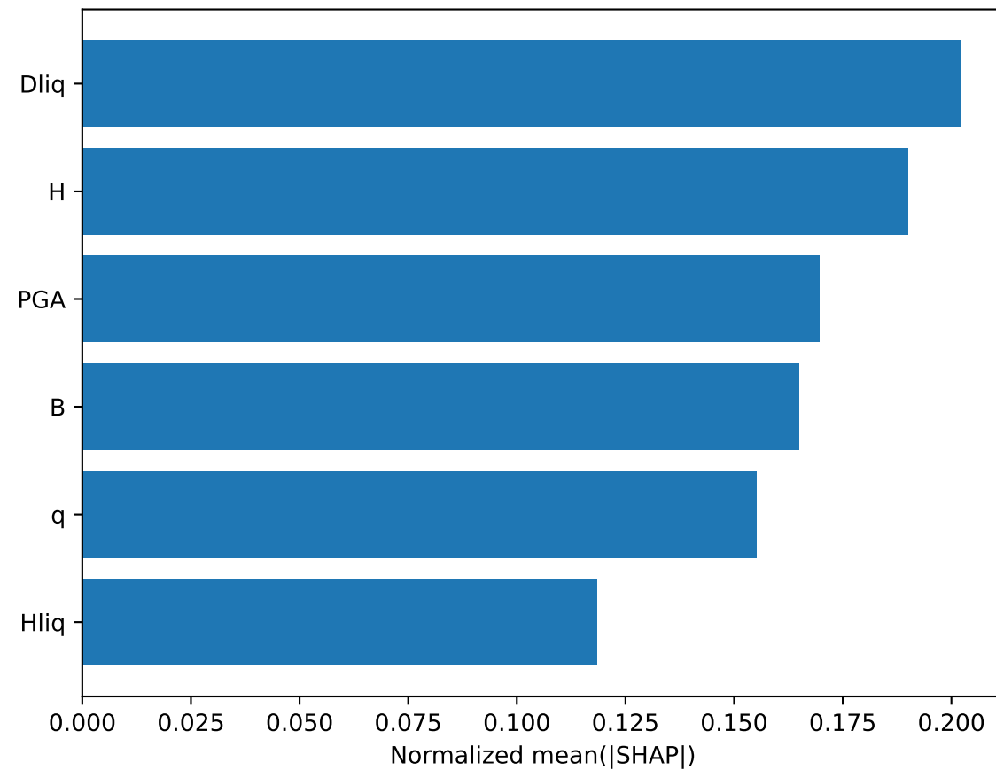
RandomForest
