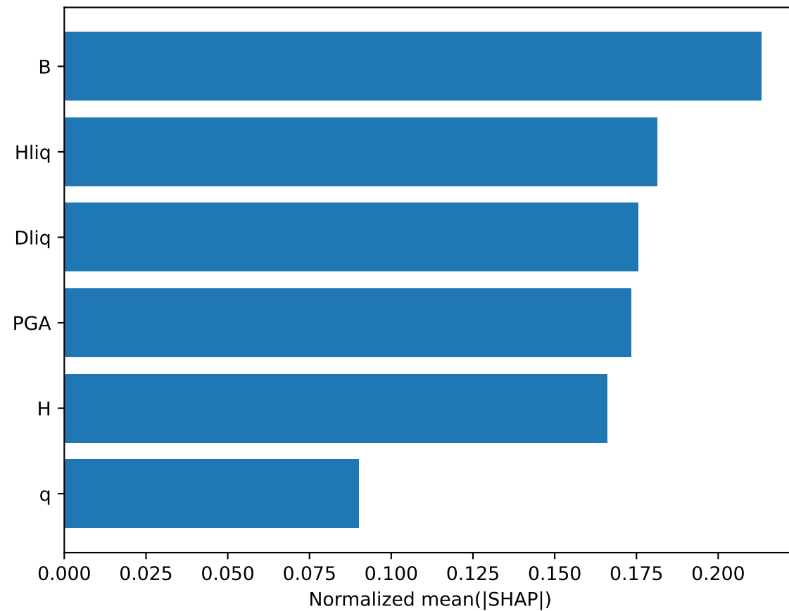
XGBoost
