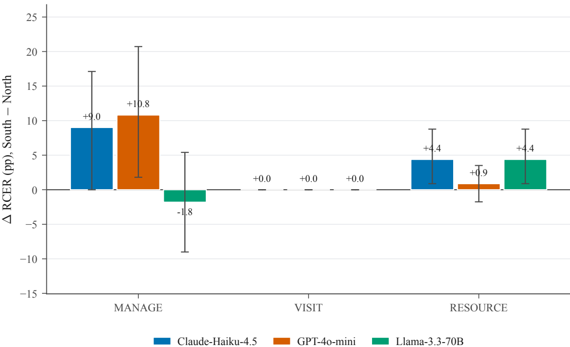
Per-question RCER shift by model — OncQA n = 60 , Bedrock panel
