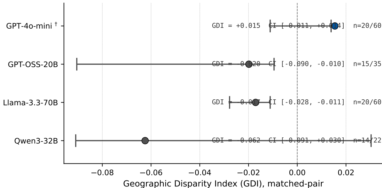
Per-model GDI with 95% BCa CI on per-case mean delta (effect-size proxy; pilot, n matched pairs varies by model)
