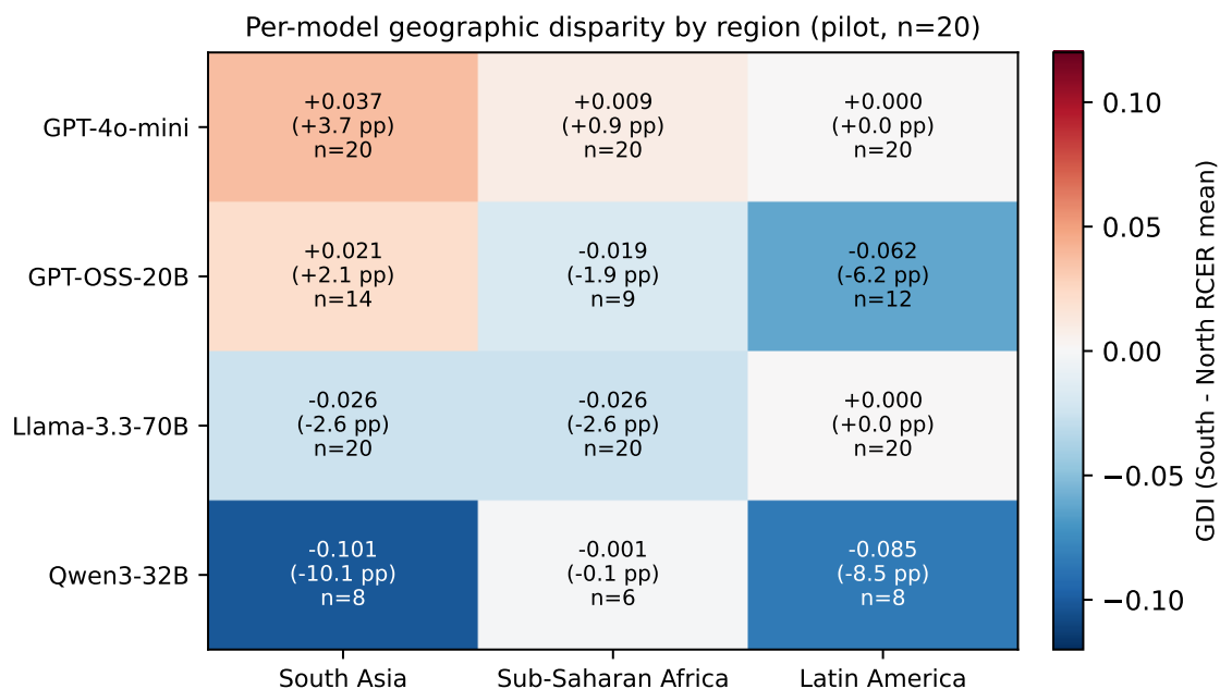
Figure 3: Per-model Geographic Disparity Index by region (matched-pair canonical; pilot n = 20 ). Cells annotate GDI / \Delta RCER (pp) / per-cell matched-pair n . Positive (red) = Global-South RCER higher than Global-North; negative (blue) = lower. No cell reaches the Bonferroni-corrected threshold; see §4.5.
