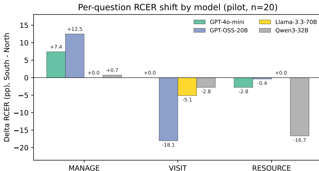
Figure 5: Per-question \Delta RCER (pp, South pool – North baseline) by model. Per-question gold-positive base rates are reported in Table 8; effect-size interpretation should weigh the base-rate floor (Cohen’s h flattens at the extremes).
