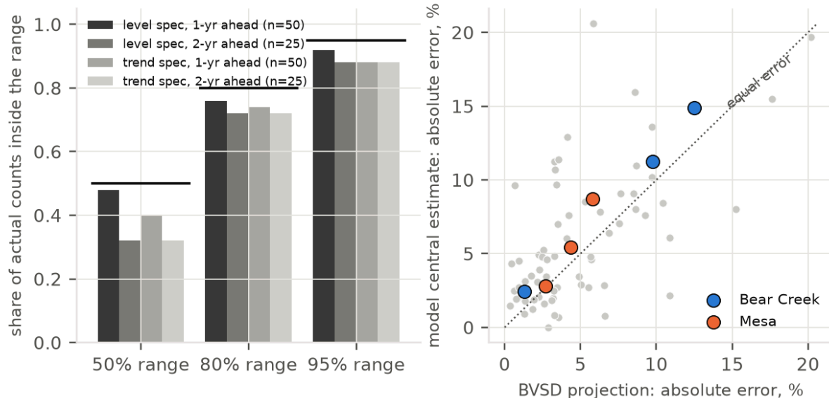
Share of actuals inside each range, 26 schools (black tick = the share the range is designed to contain) Standard school-years, trend spec: model vs BVSD
