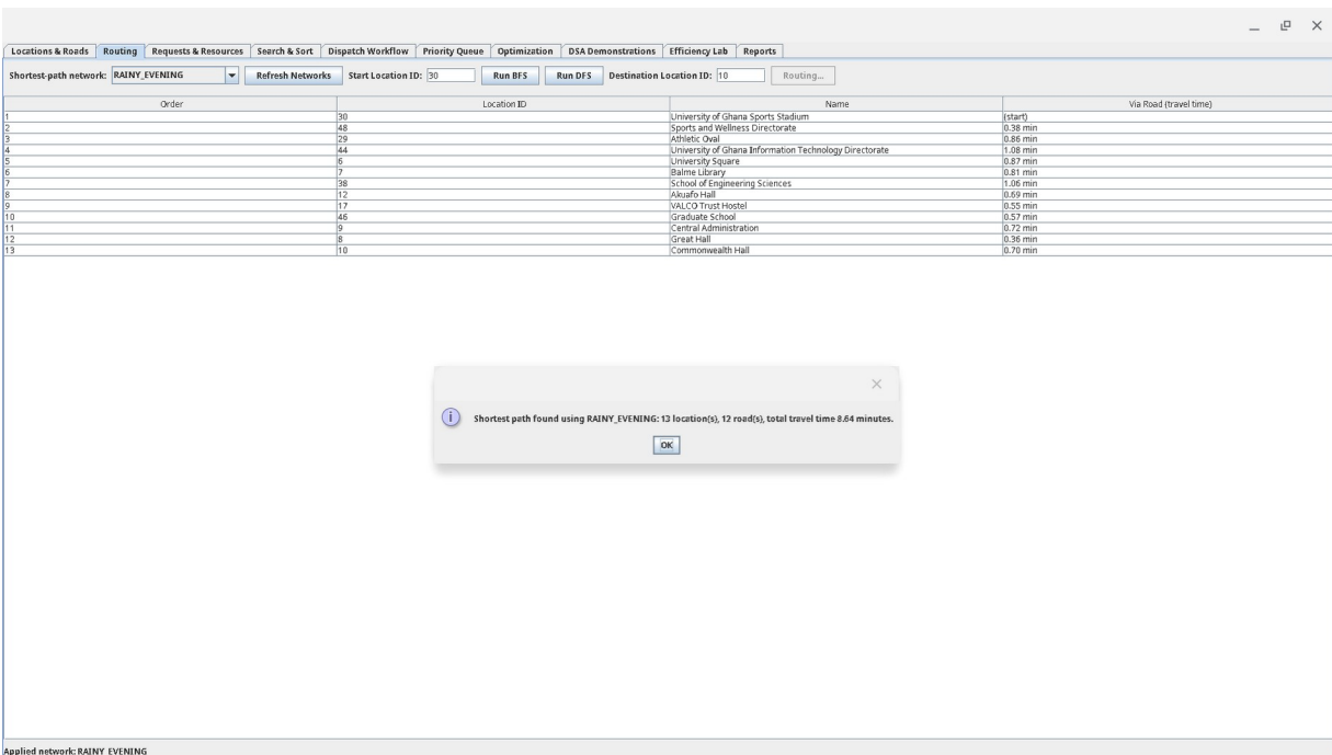
Figure 7. Dijkstra shortest path from the UG Sports Stadium to Commonwealth Hall under the RAINY_EVENING scenario; modeled travel cost: 8.64 minutes.
