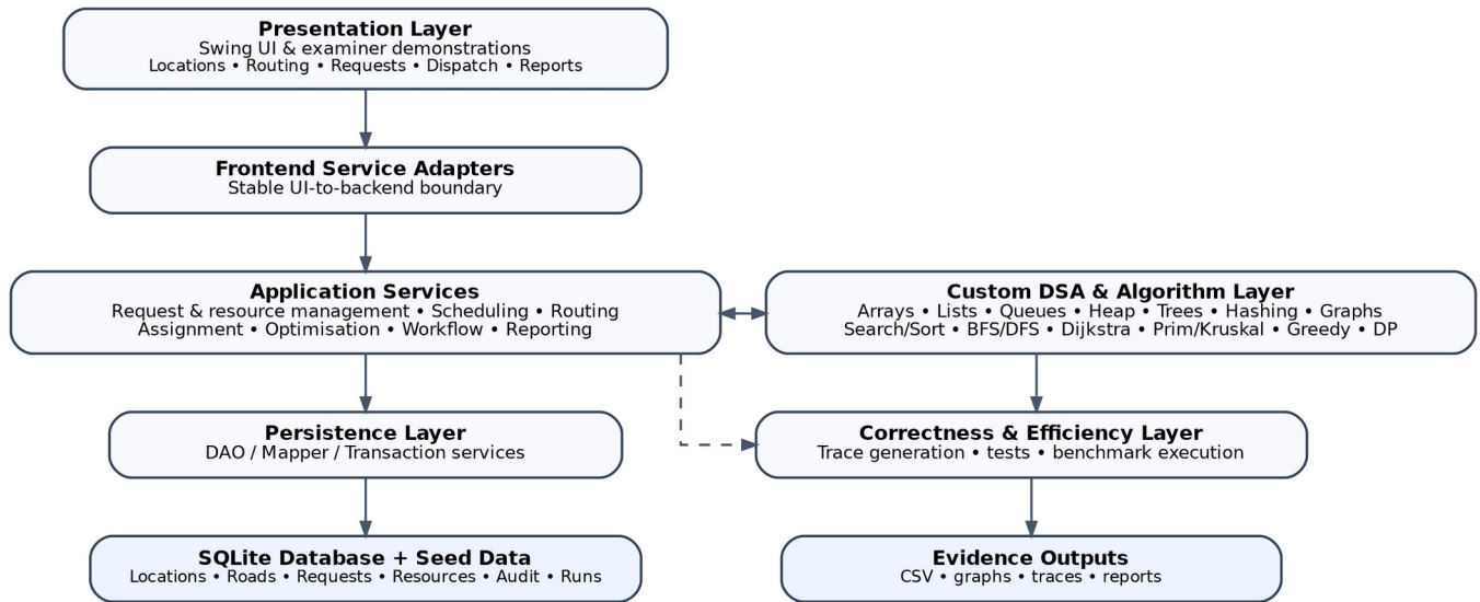
Figure 2. Layered architecture and operational/evidence flow of the integrated system.
