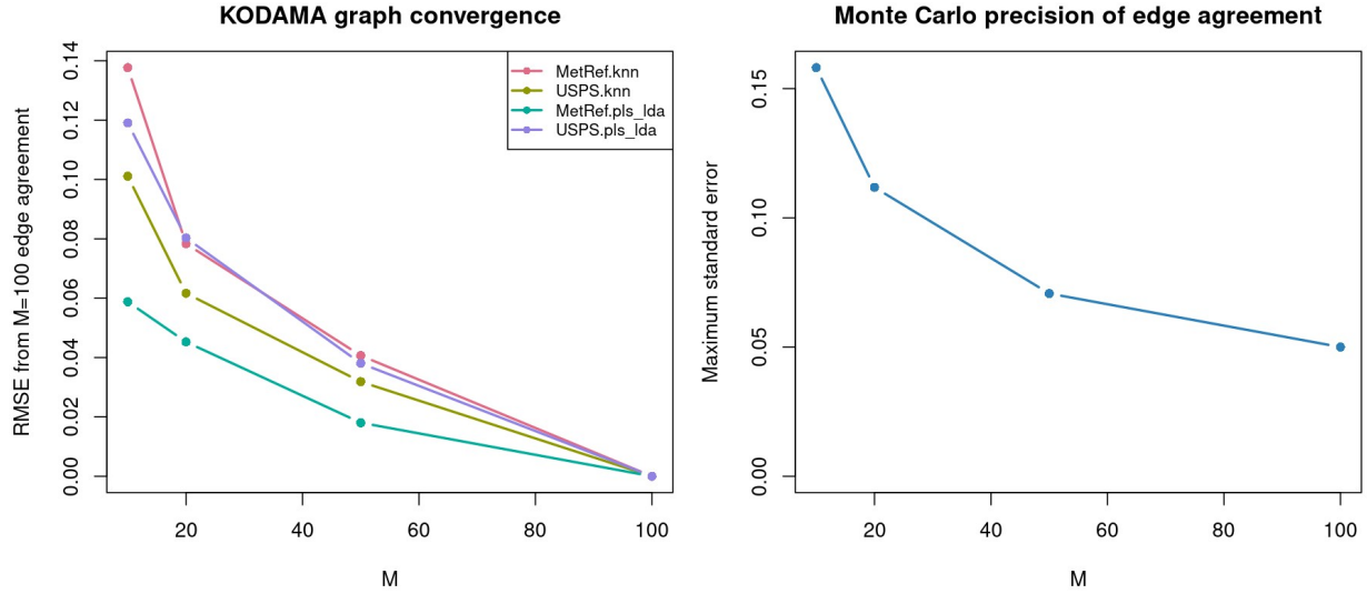
Figure 4. Convergence of edge-agreement weights as independent KODAMA runs are added. RMSE is measured against the M = 100 ensemble; the right panel shows the Bernoulli worst-case Monte Carlo standard error.
