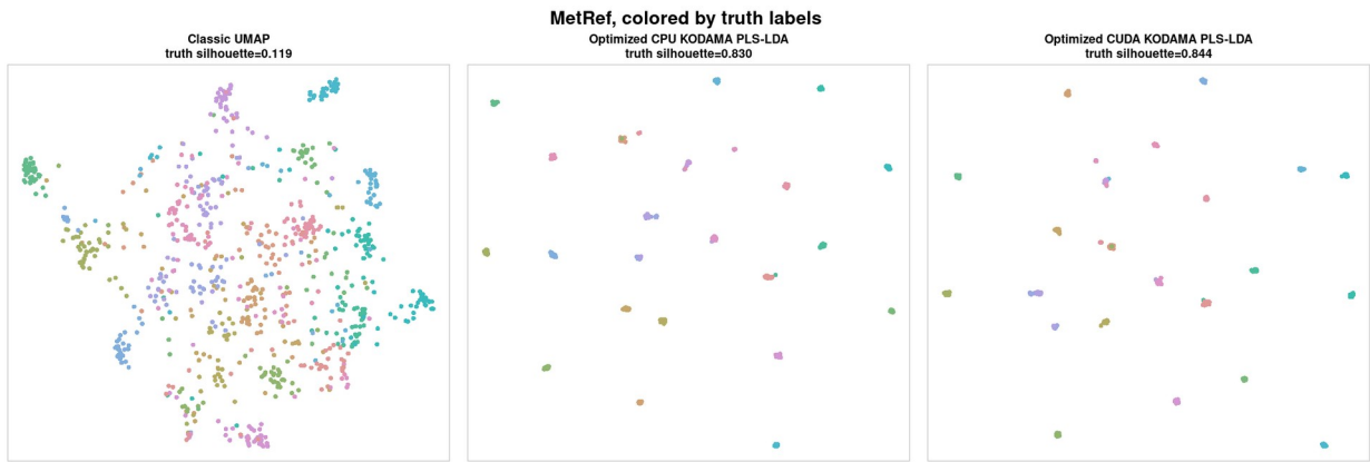
Figure 2. Matched MetRef UMAP validation after the float32 PLS-LDA optimization. Classic data, CPU KODAMA, and CUDA KODAMA use exact k = 30 , the same original-data PCA initialization, seed, epochs, and CPU embedding implementation. Colors are external reference labels withheld from optimization.
