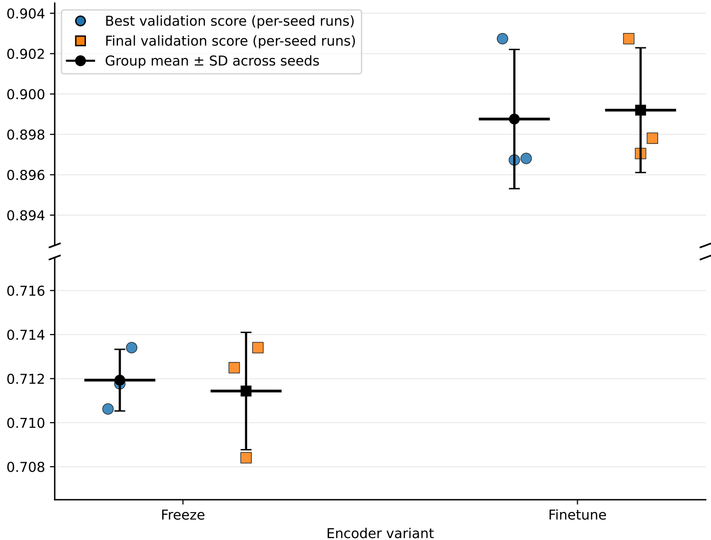
Validation hard@0.5 score
