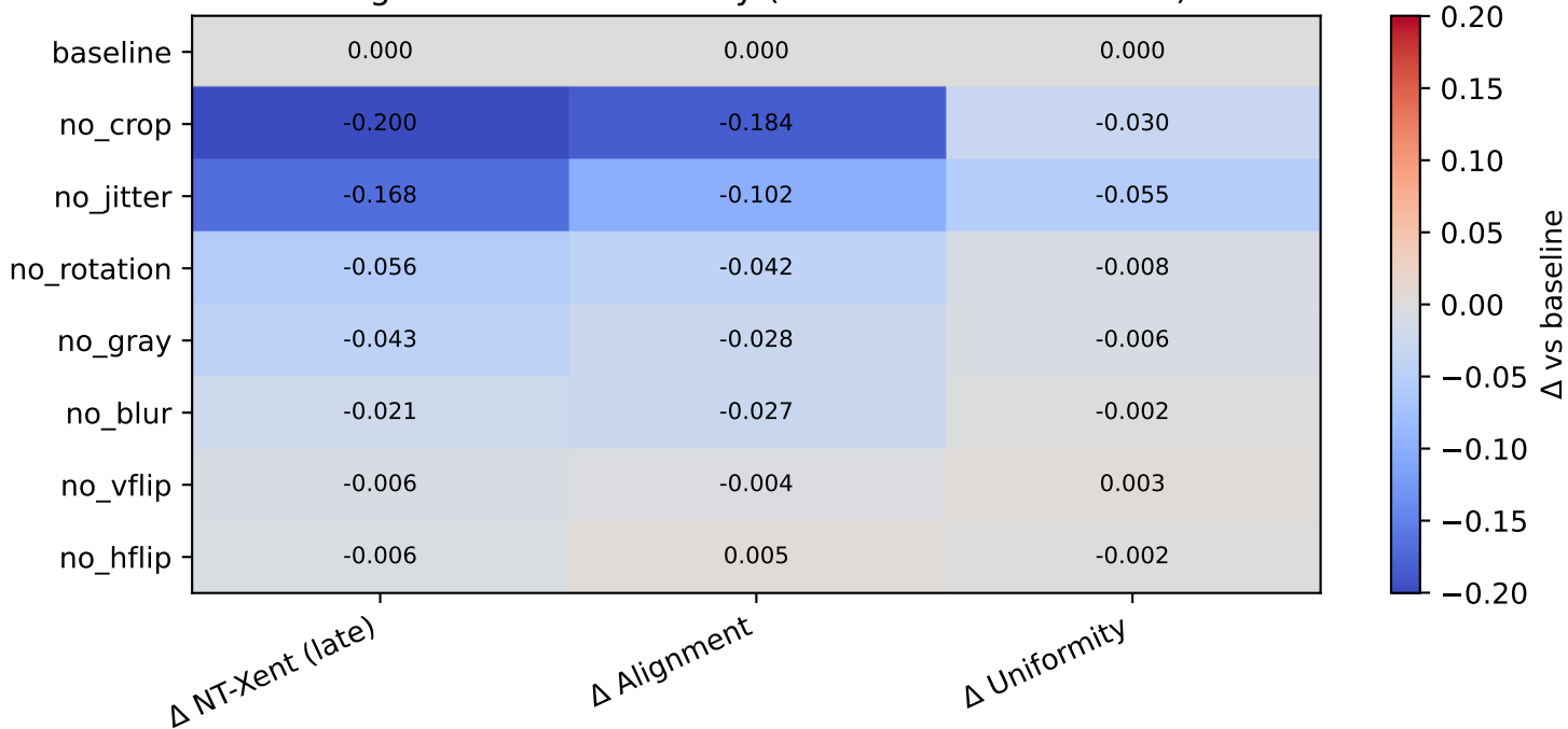
Augmentation sensitivity ( \Delta vs baseline: baseline)
