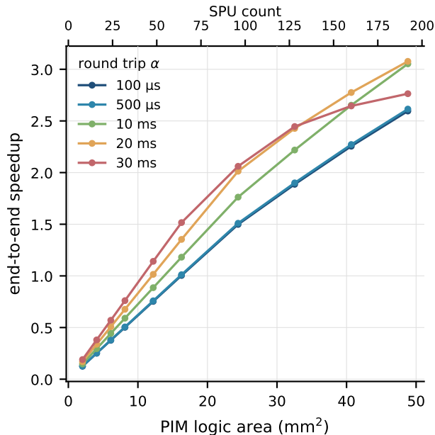
L40S — 24 ch ceiling (192 SPU)
