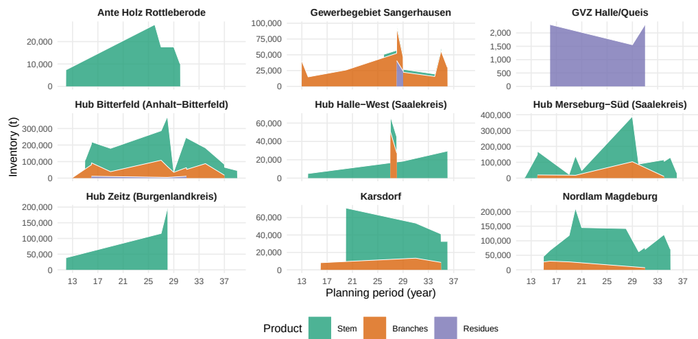
Figure 15: End-of-period inventory levels at storage/pre-treatment hubs, disaggregated by product type. Each panel corresponds to one active hub.
