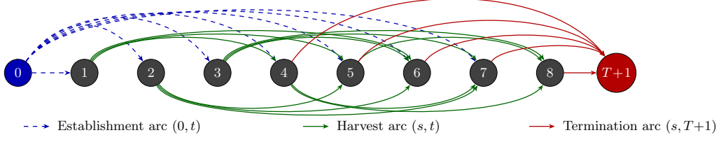
Figure 4: Network structure of set \mathcal{S} for T = 8 , A_{\min} = 3 , A_{\max} = 5 . Dashed blue arcs: establishment arcs (0, t) , t \in \{1, \dots, T-1\} . Solid green arcs above: harvest arcs (s, t) with odd s ; below: harvest arcs with even s . Solid red arcs: termination arcs (s, T+1) , s \in \{A_{\min} + 1, \dots, T\} .
