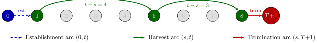
Figure 5: Example of a feasible path through the network for T = 8 , A_{\min} = 3 , A_{\max} = 5 : establishment in period 1, harvests in periods 5 and 8, termination at T + 1 .
