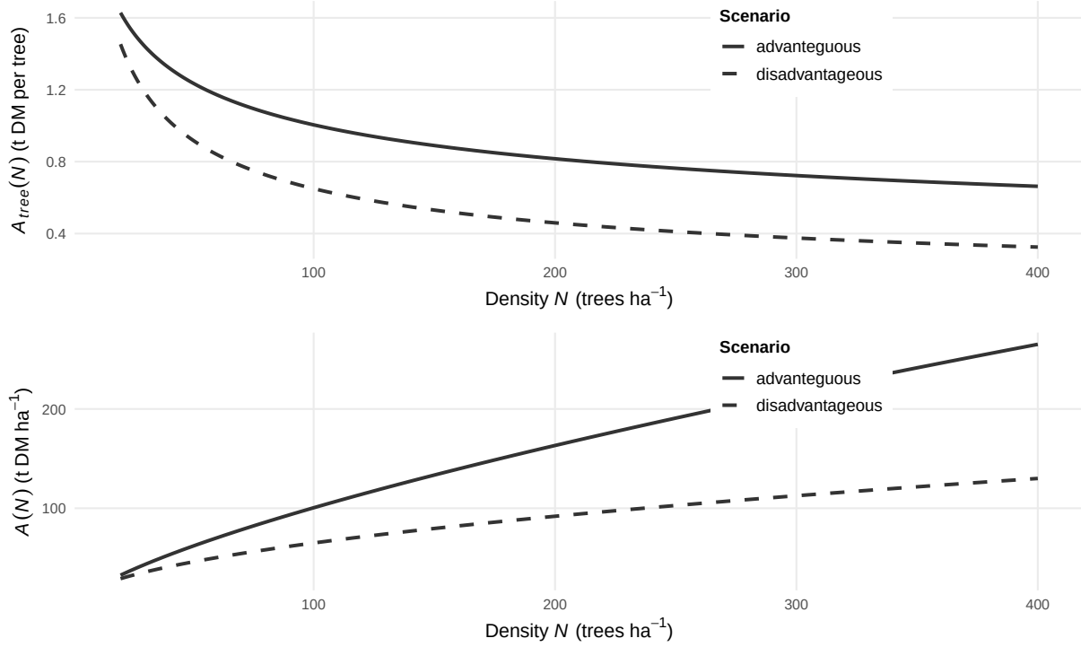
FIGURE 2 Tree-level and stand-level Gompertz asymptote functions A_{\text{tree}}(N) and A(N) for advanteguous ( N = 4 , \beta = -0.3 ) and disadvantageous ( N = 6.5 , \beta = -0.5 ) site conditions.
