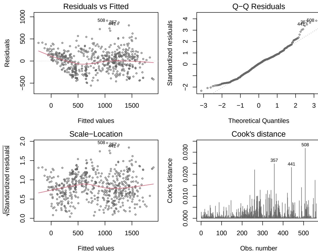
Figure 15: OLS-Diagnostik: Residuen vs. Fitted, Q-Q-Plot, Scale-Location und Cook's Distance.
