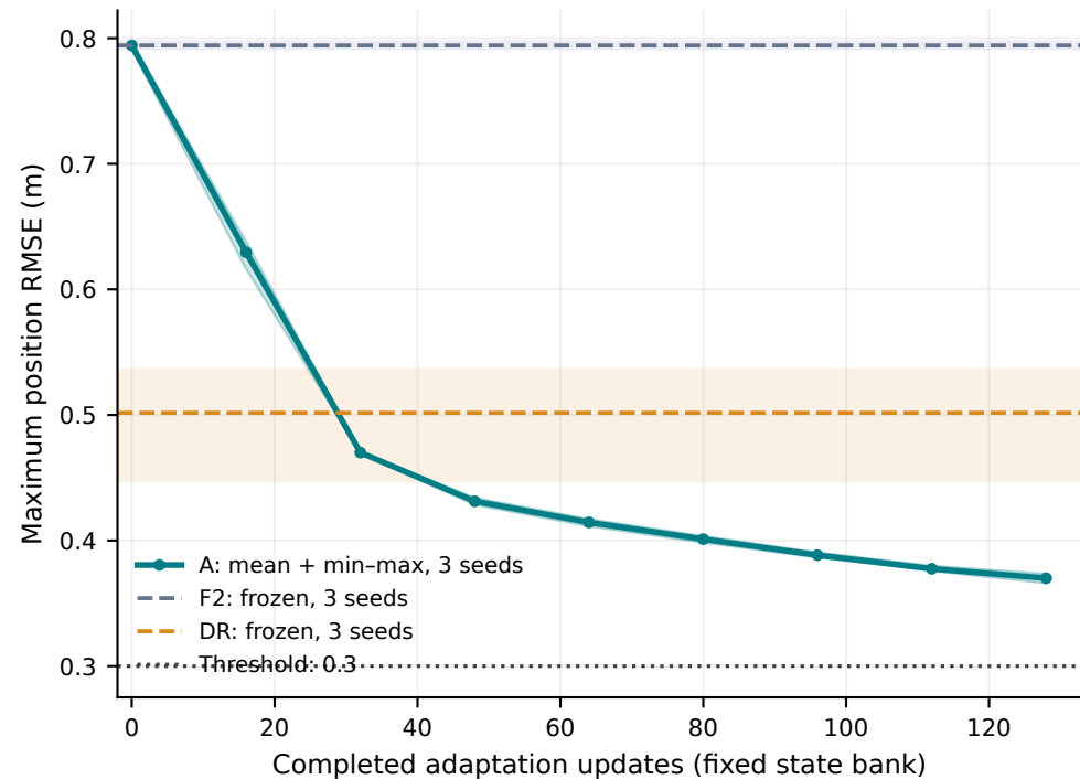
Combined fault · 3/3 seeds censored at 128 updates
