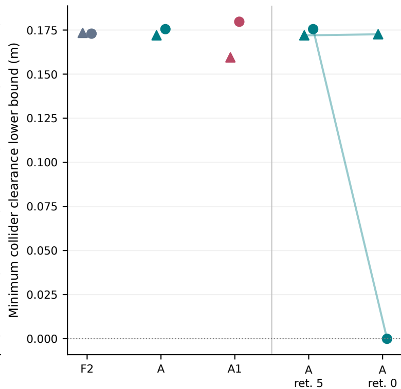
B. Two validation worlds · seed 11
