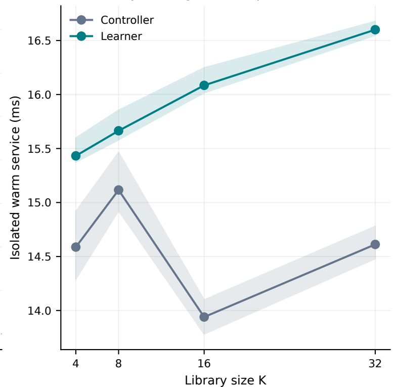
C. Cost only · changed-K competence unavailable
