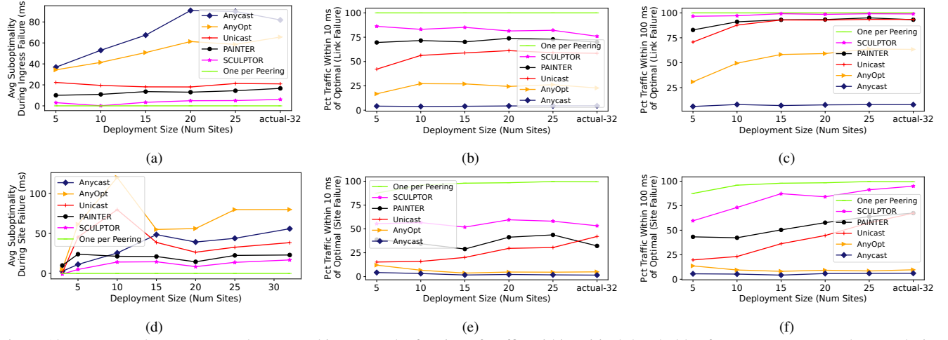
Figure 10: SCULPTOR lowers average latency and increases the fraction of traffic within critical thresholds of One-per-Peering latency during both link and site failures over many emulated deployments.
