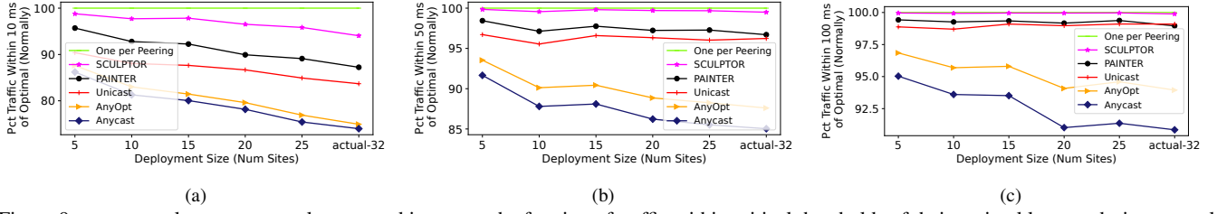
Figure 9: SCULPTOR lowers average latency and increases the fraction of traffic within critical thresholds of their optimal latency during normal operation.
