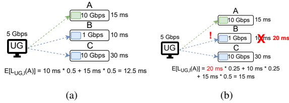
Figure 8: A UG has a path to two prefixes, green and blue. The green prefix is only advertised via ingress A and the blue prefix is advertised via two ingresses B and C, each of which are equally likely for this UG. If the UG prefers B over C, we assign the client to the blue prefix (10 ms) while if the UG prefers C over B we will assign the client to the green prefix (15 ms). Hence the initial expected latency is the average of 10 ms and 15 ms corresponding to whether this UG prefers ingress B or C (8a). However, ingress B does not have sufficient capacity to handle this UG's traffic and so is congested with 50% probability corresponding to the 50% probability that this user prefers ingress B. We artificially inflate this UG's expected latency (and all other UG's using ingress B) to reflect this possible overutilization (8b).
