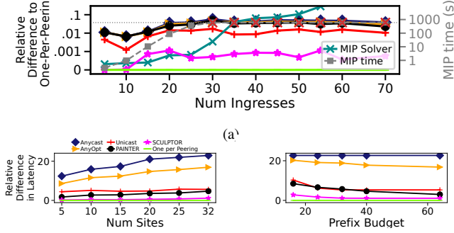
Figure 7: Microevaluations. (a) Sub-optimality of the latency+MLU objective relative to the one-per-peering bound as the deployment grows one ingress at a time (5 deployments per size; legend as in (b)) against the full advertisement MIP (HiGHS, 10-minute budget), whose solve time is the gray dashed line on the right axis; steady-state latency sub-optimality vs. number of sites (b) and prefix budget (c).
