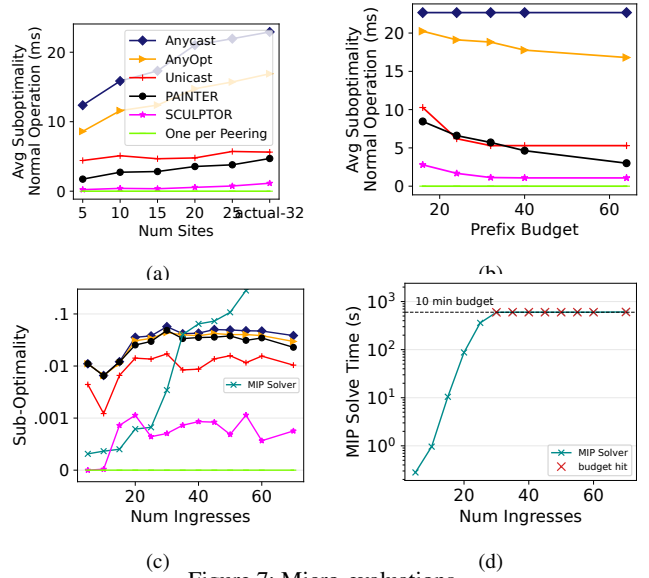
Figure 7: Micro-evaluations.
