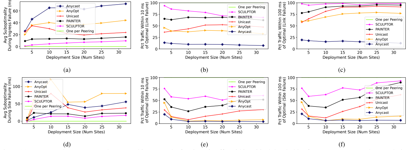
Figure 11: SCULPTOR lowers average latency and increases the fraction of traffic within critical thresholds of One-per-Peering latency during both link and site failures over many emulated deployments.
