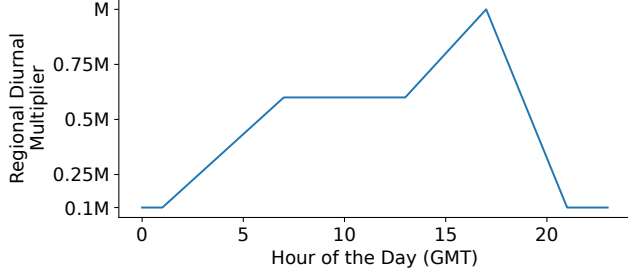
Figure 8: The diurnal traffic shape we apply in Section 5.3.2, taken from prior work [20].
