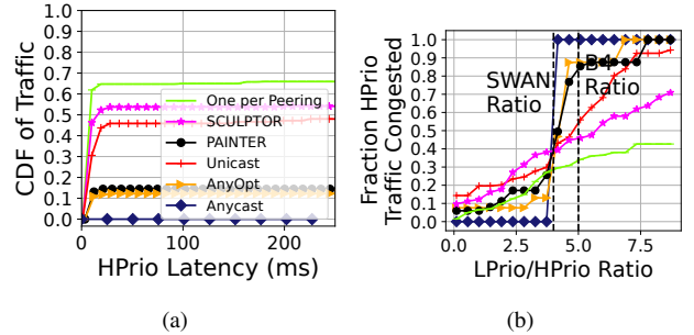
Figure 6: SCULPTOR routes high-priority traffic with low latency (6a) and minimal congestion from low-priority traffic (6b). We inferred L_{Prio}/H_{Prio} ratios for SWAN [18] and B4 [17] from those papers.
