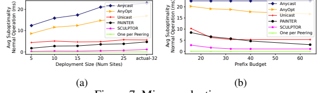
Figure 7: Micro evaluations.
