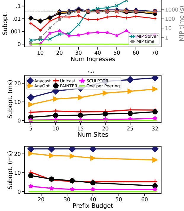
Figure 7: Micro-evaluations. (a) Sub-optimality of the latency+MLU objective relative to the one-per-peering bound as the deployment grows one ingress at a time (5 deployments per size; legend as in (b)) against the full advertisement MIP (HiGHS, 10-minute budget), whose solve time is the gray dashed line on the right axis; steady-state latency sub-optimality vs. number of sites (b) and prefix budget (c).
