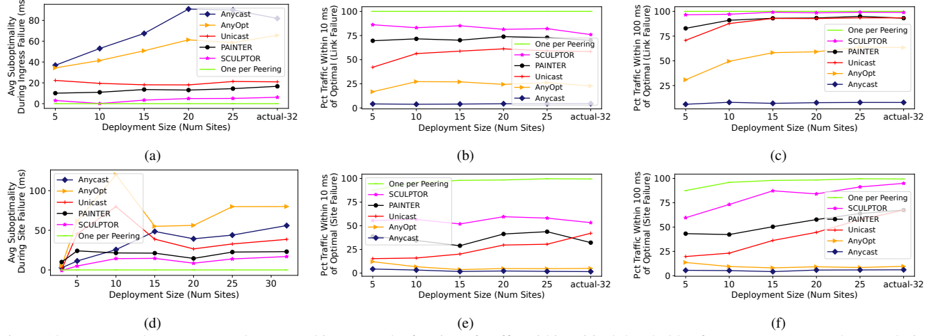
Figure 10: SCULPTOR lowers average latency and increases the fraction of traffic within critical thresholds of One-per-Peering latency during both link and site failures over many emulated deployments.
