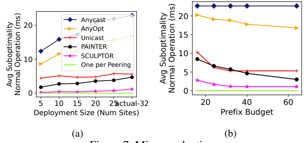
Figure 7: Micro evaluations.
