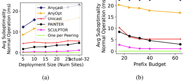
(a) Figure 7: Micro evaluations.
