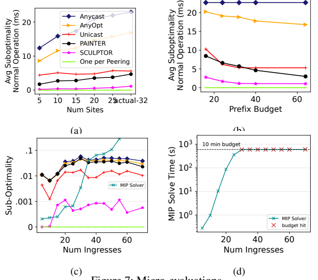
Figure 7: Micro-evaluations.
