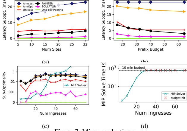
Figure 7: Micro-evaluations.
