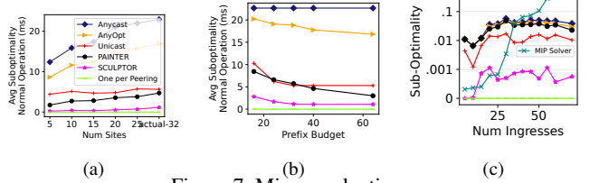
Figure 7: Micro evaluations.
