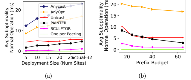
Figure 7: Micro evaluations.
