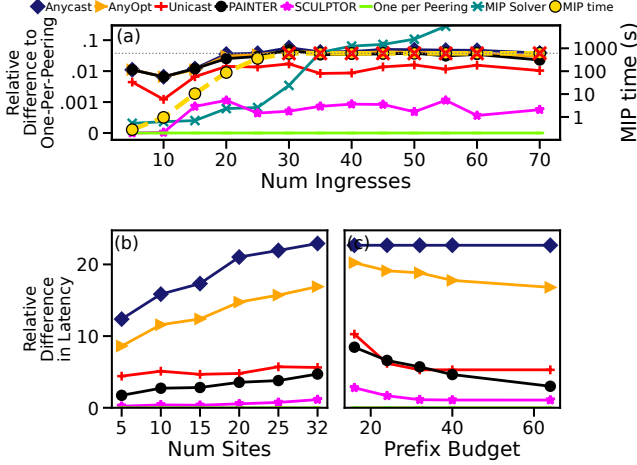
Figure 7: Micro-evaluations. (a) Sub-optimality of the latency+MLU objective relative to the one-per-peering bound as the deployment grows one ingress at a time (5 deployments per size) against the full advertisement MIP (HiGHS, 10-minute budget), whose solve time is the gold dashed line on the right axis (x: budget hit); steady-state latency sub-optimality vs. number of sites (b) and prefix budget (c).
